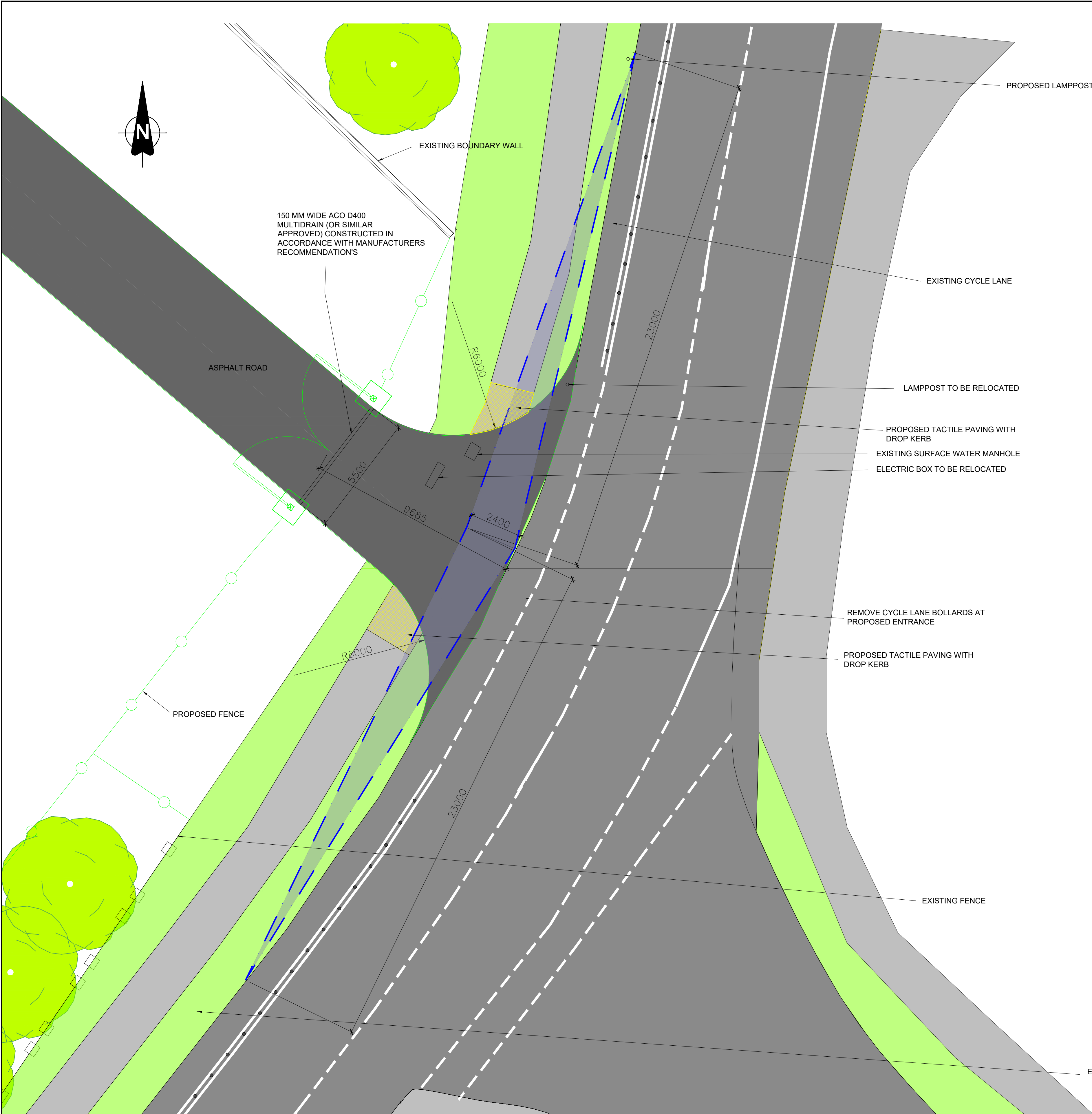
ROAD ENTRANCE SCALE 1:100
